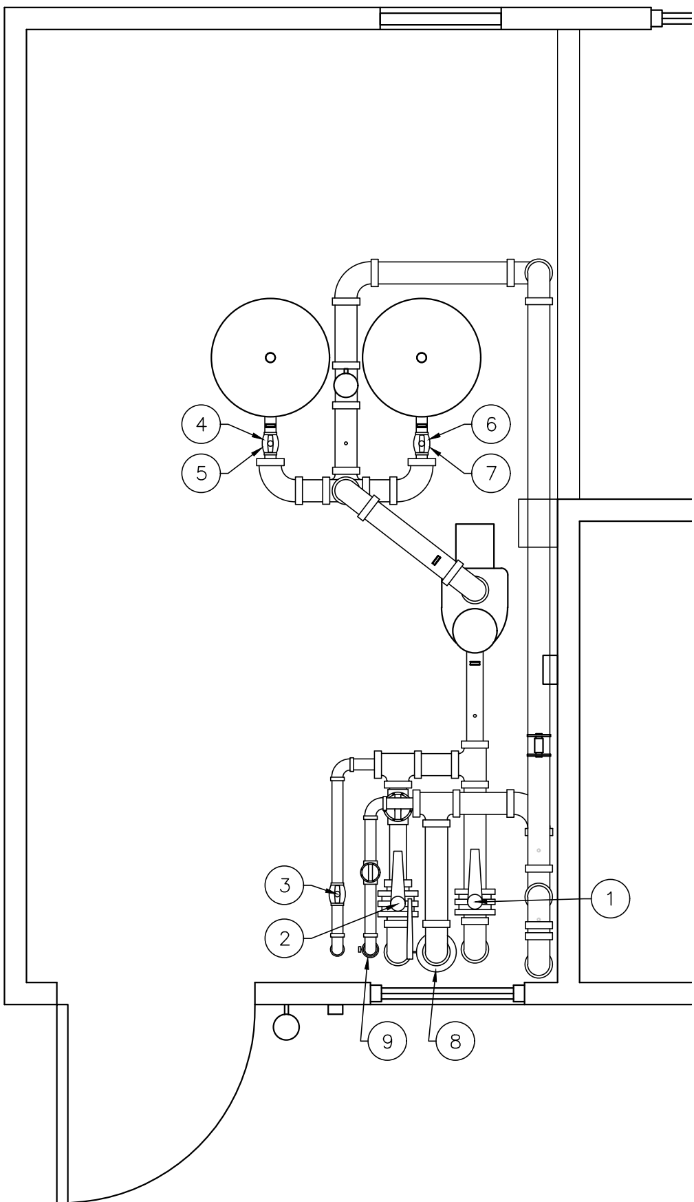
SWIMMING POOL #2 MECHANICAL ROOM VALVE DIAGRAM N.T.S.
